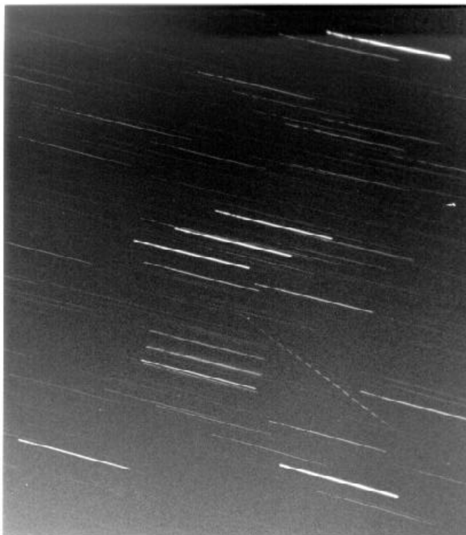
Foto 3 : Leonide magnitude -2 in Orion. Woignarue, 17 november 1996 3h57m14s UT.
