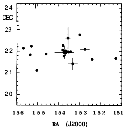
Fig. 1. Geocentric radiant positions, Leonids 1995 DMS. Radiant positions have been corrected for radiant drift to November 18, 0 h UT and radiants from trajectories with a Q angle smaller than 11 have been removed. A radiant concentration at RA = 153.63 ; DEC = +21.97 is obvious
